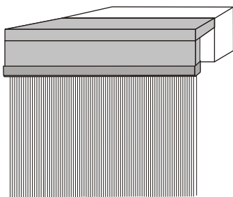
AQUA RAIN Part # G A 0 3 _____ 48 OR 64 STREAMS PER LIN FT. 2 ROW VERTICAL WATER DIRECTION RATE: 1/2 OR 2/3 G.P.M. PER INCH REMOVABLE NOZZLE INSERTS FOR DEBRIS
