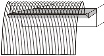
AQUA WAVE SSR Part # G A 0 5 _____ 48 STREAMS PER LIN. FT. SINGLE ROW ARC OF WATER RATE: 1 G.P.M. PER INCH
